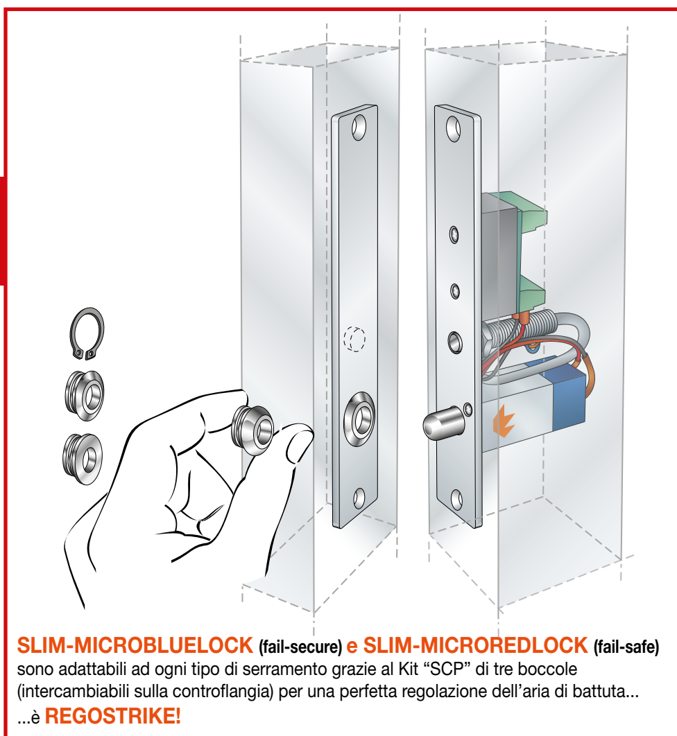
SLIM-MICROREDLOCK (fail-safe)
